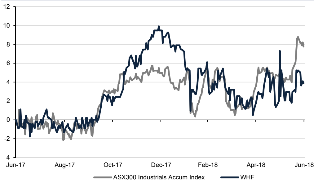
FIG.117: WHF TSR V ASX 300 INDUSTRIALS ACCUMULATION INDEX
