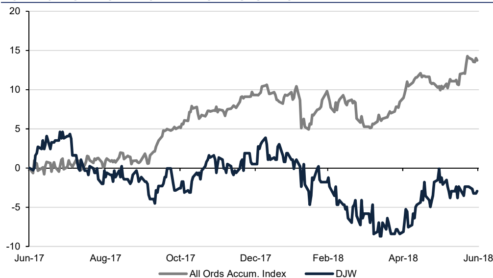
FIG.41: DJW TSR V ASX ALL ORDINARIES ACCUMULATION INDEX
