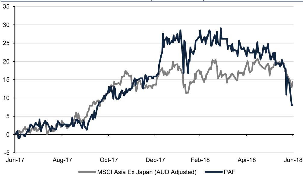
FIG.81: PAF TSR V MSCI ASIA EX JAPAN INDEX (AUD ADJUSTED)
